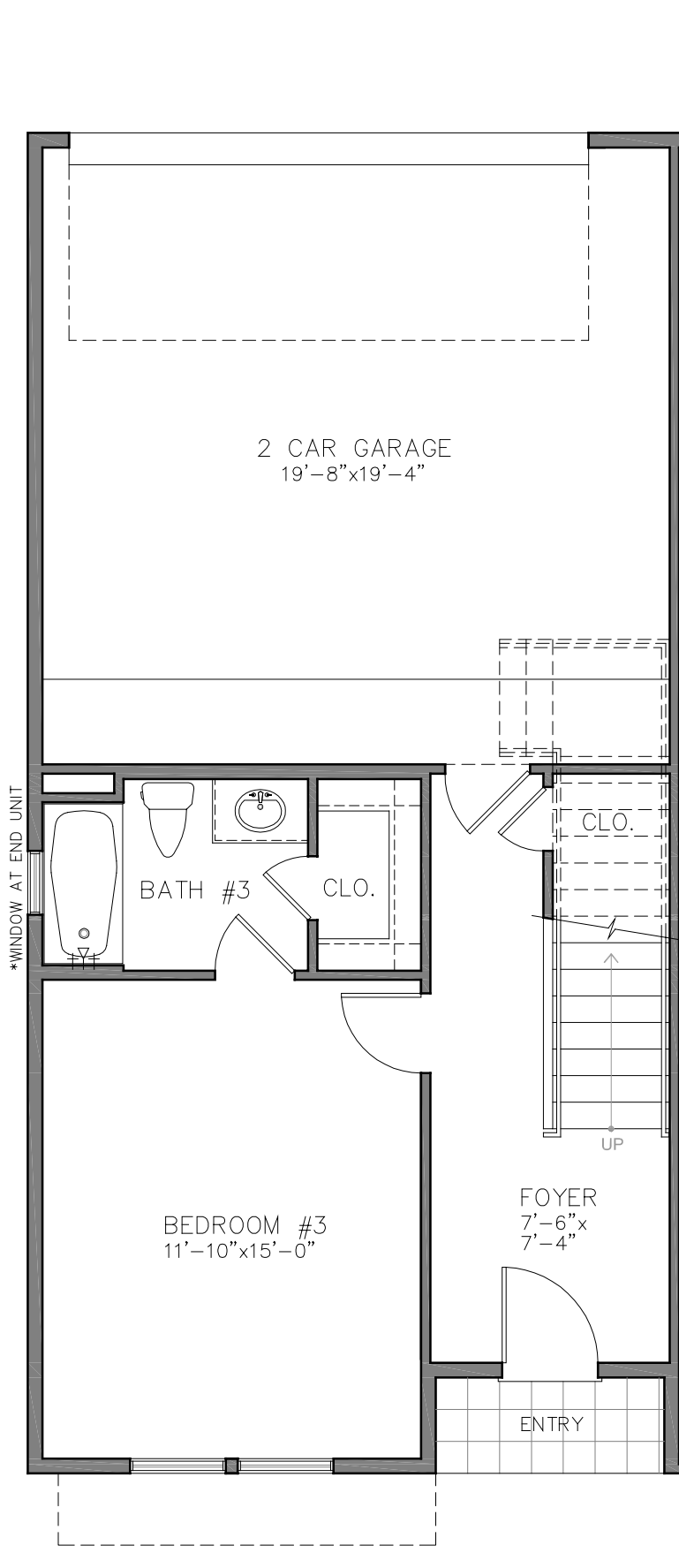
DELANO-2070 GROUND FLOOR PLAN
