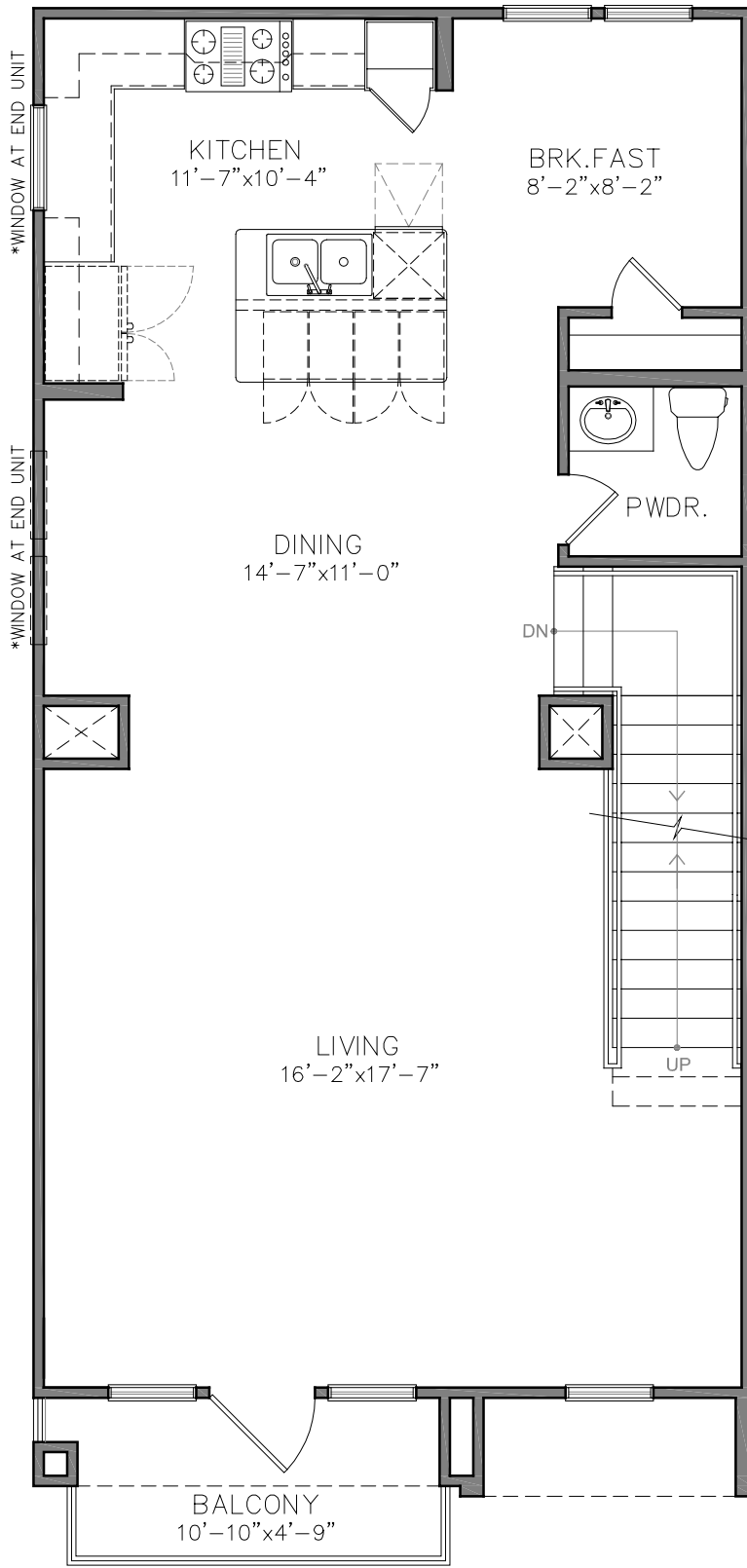
DELANO-2070 SECOND FLOOR PLAN
