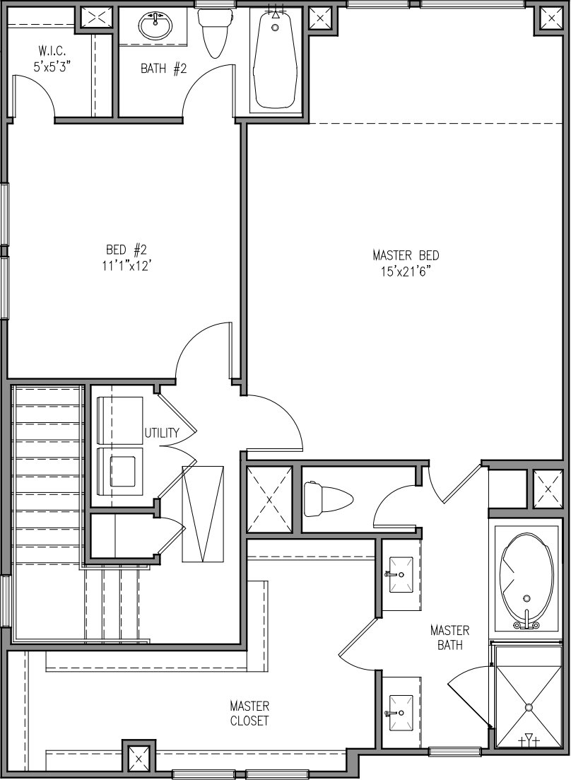
3RD FLOOR PLAN
